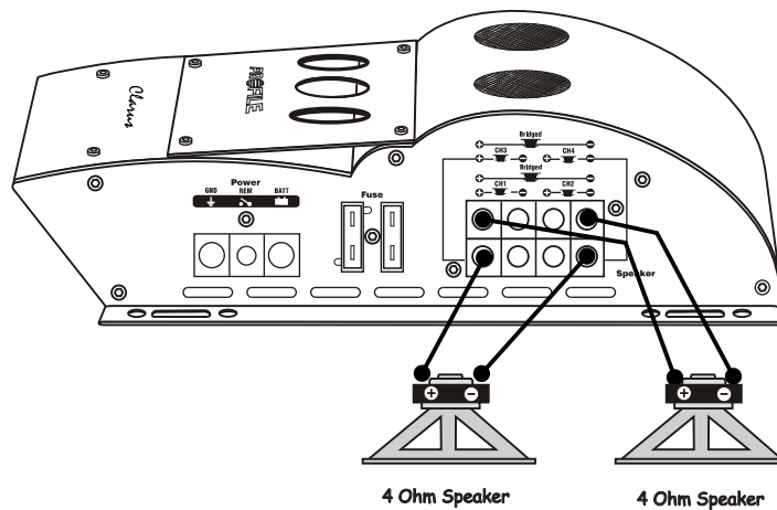
FOUR CHANNEL BRIDGED SPEAKER CONNECTIONS
